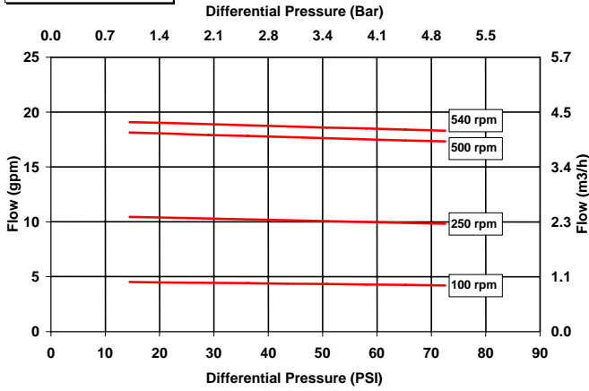
C8 4634 SSU (1000 cst)
