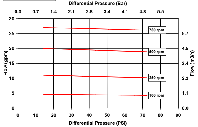
C8 2317 SSU (500 cst)
